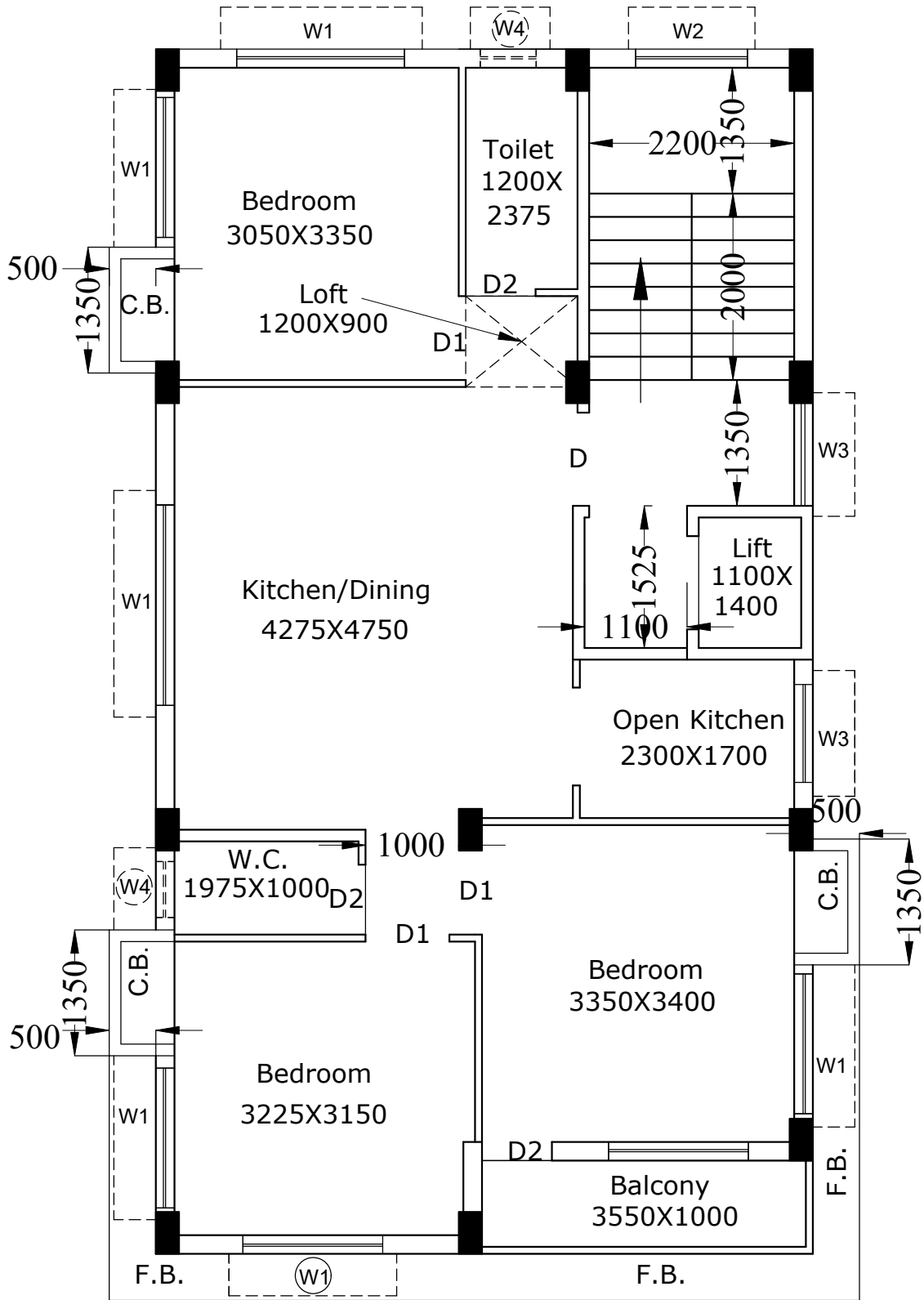
TYPICAL FLOOR PLAN 1ST,2ND & 3RD FLOOR
